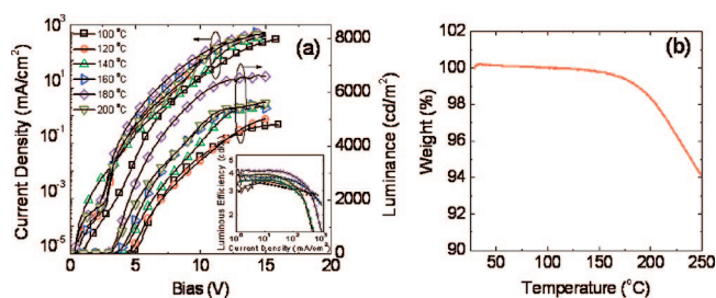
Figure 4. (a) The J-L-V characteristics of device C with QDs having been annealed at different temperatures for 10 min. The inset of (a) shows the corresponding luminous efficiency versus current density curves. (b) Thermogravimetric analysis of CdSe/CdS/ZnS core/shell/shell QDs on the ITO/PEDOT/poly-TPD/DNA-CTMA multilayer.
